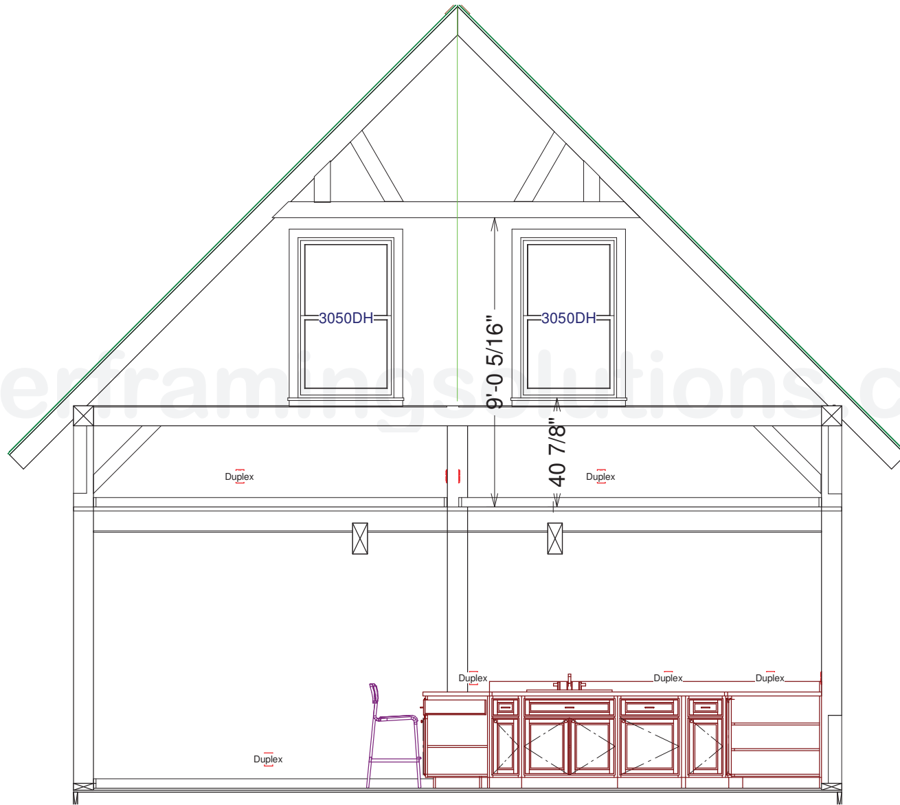
LOFT WINDOW ELEVATION
